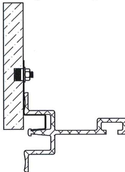
Installed fastener (Section A - A)
