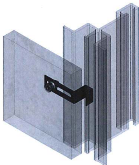
Installed fastener (3D view)
